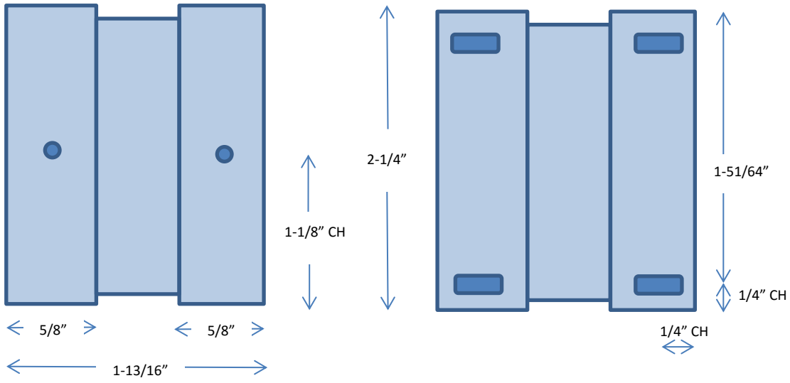
2 Holes – 5/32" D
